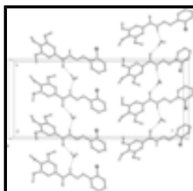
Fig. 2. The packing of (I), viewed down the b axis. The dashed lines represent the hydrogen bonding interactions.
