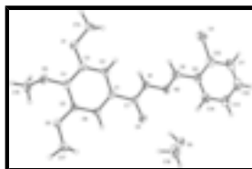
Fig. 1. The molecular structure of (I) with displacement ellipsoids for the non-hydrogen atoms drawn at the 50% probability level.
